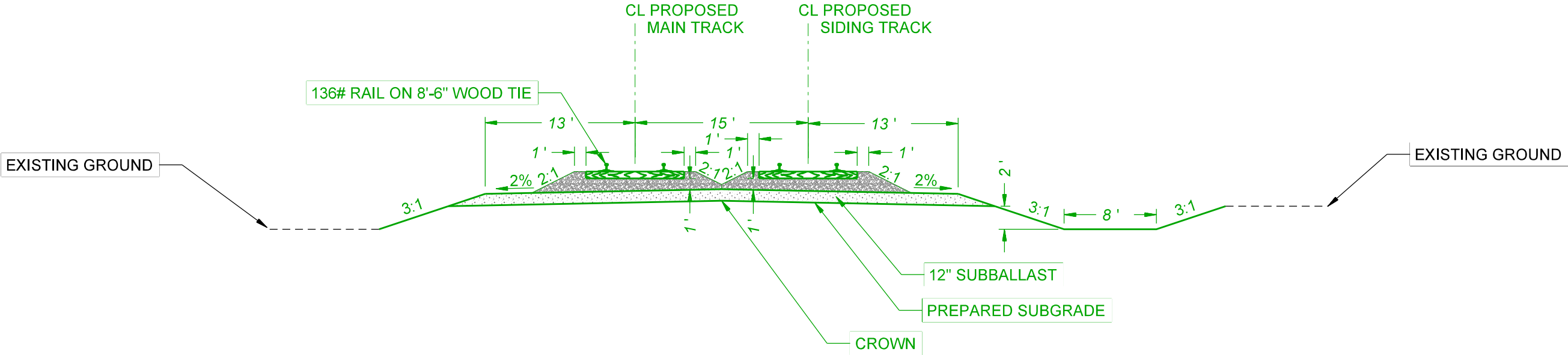
TYPICAL SECTION - SINGLE TRACK w/ SIDING
